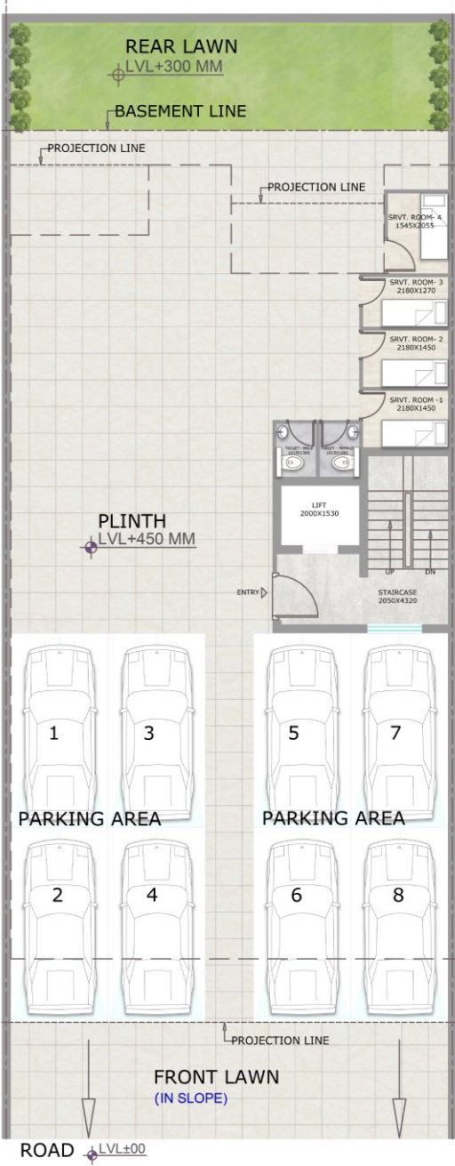
STILT FLOOR
